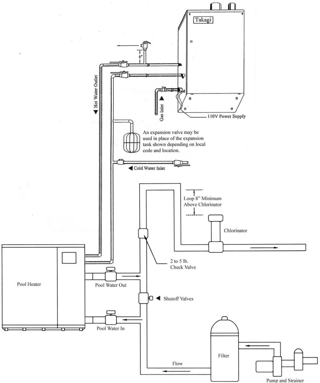
FIGURE 4 - PIPING CONNECTIONS
