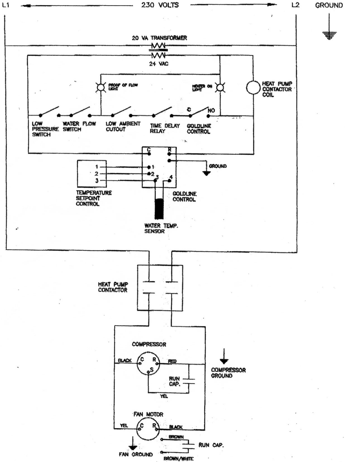
Figure 1 - Electrical Connections
